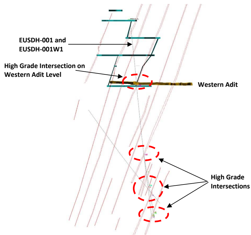
Figure 7. Oblique Section View of diamond holes EUSDH-001 and EUSDH-001W1 showing reef development
