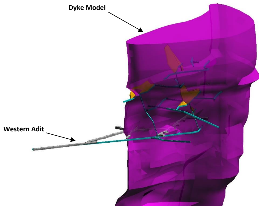
Figure 6. Isometric View of the Western Adit and Eureka Dyke Model
